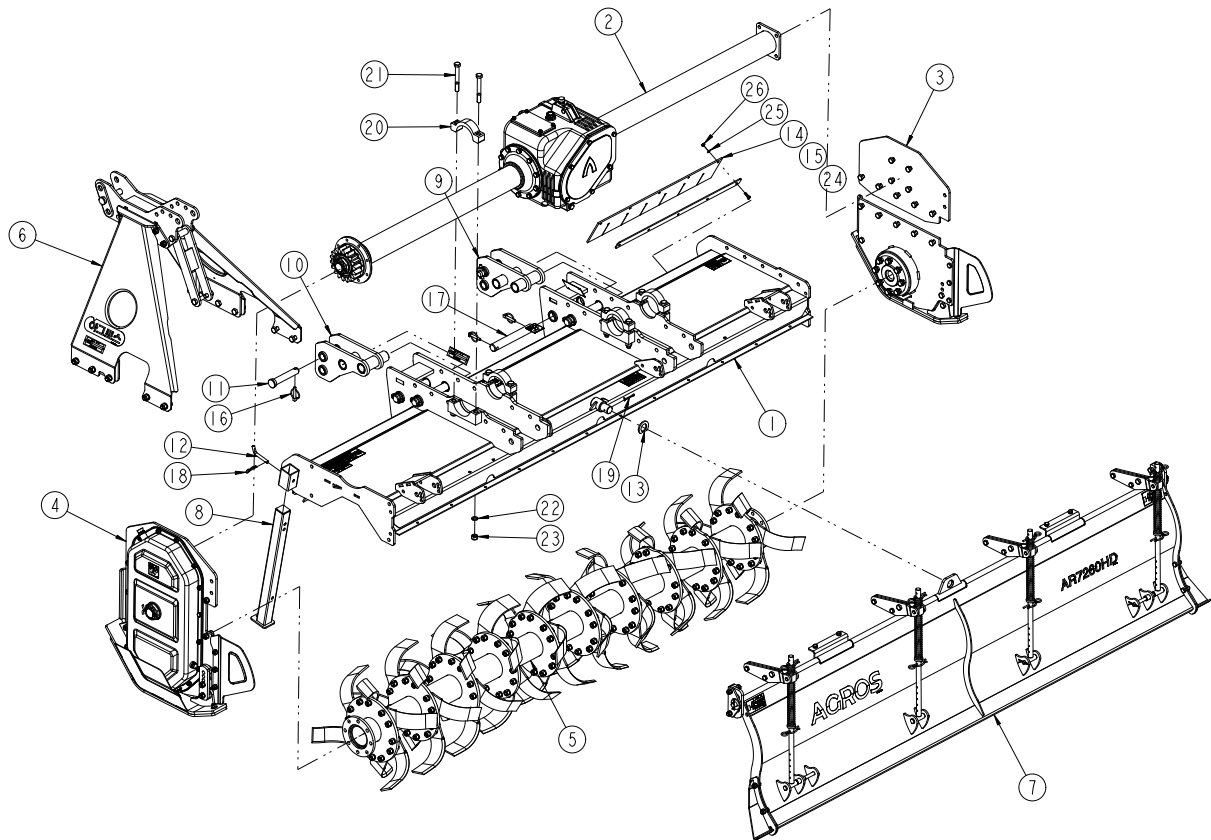
AR7260HD
