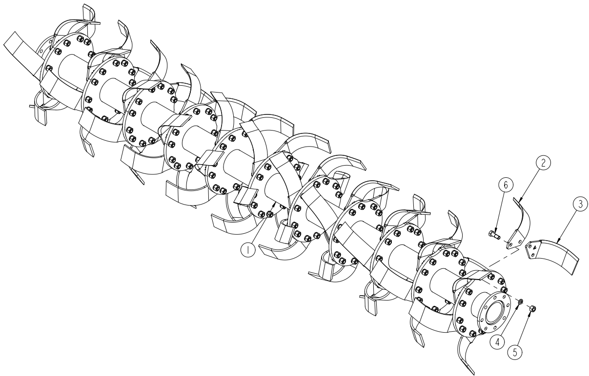
R7280-5000A
