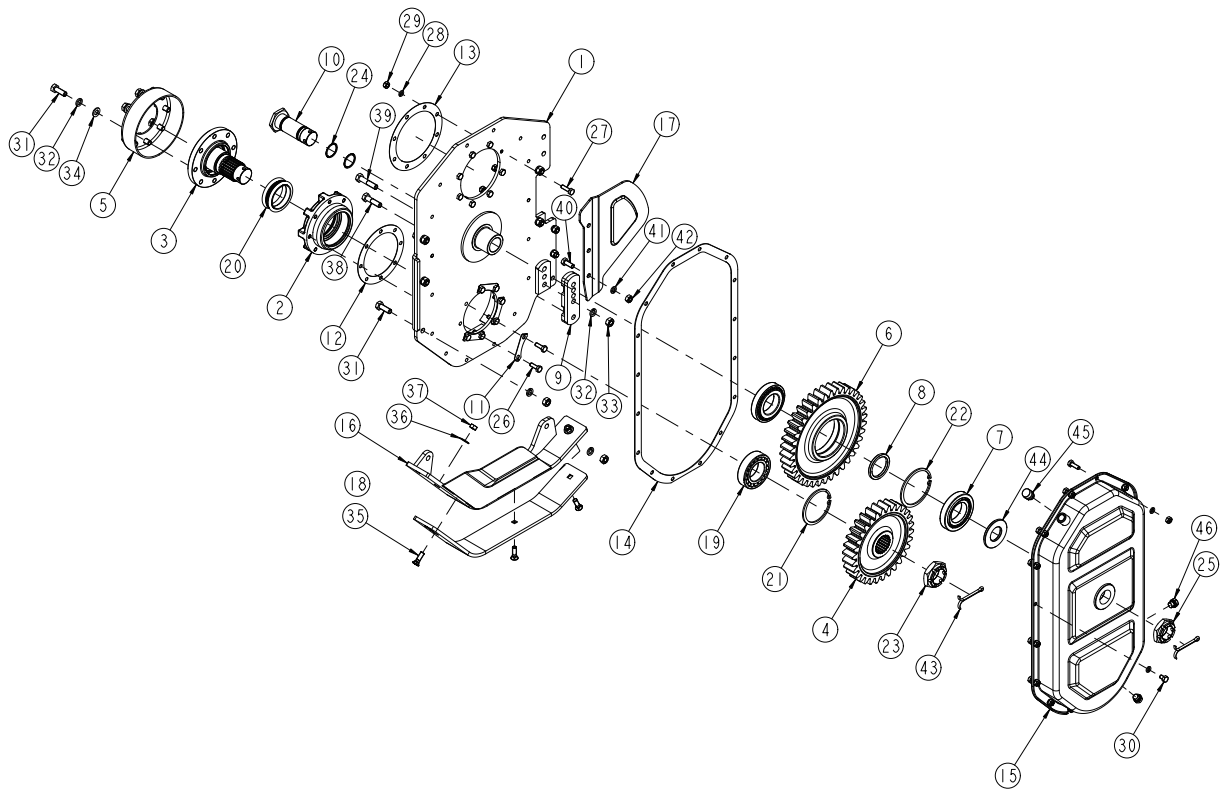
R7240-4000A
