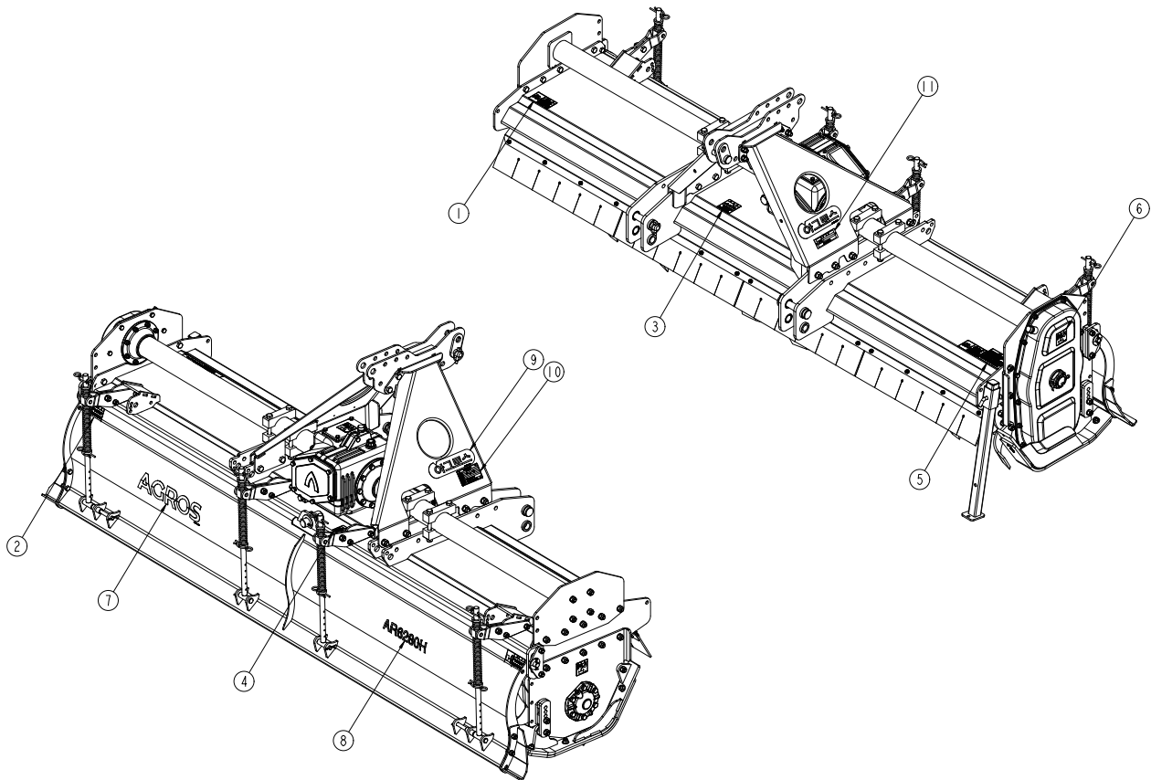
AR6280H-DECAL
